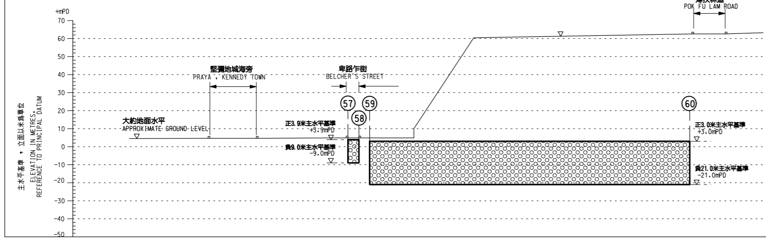
沿參線 H - H 的切面立視圖 SECTIONAL ELEVATION ALONG REFERENCE LINE H - H
