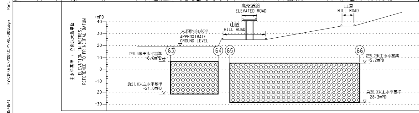
沿參線 B - B 的切面立視圖 SECTIONAL ELEVATION ALONG REFERENCE LINE B - B
