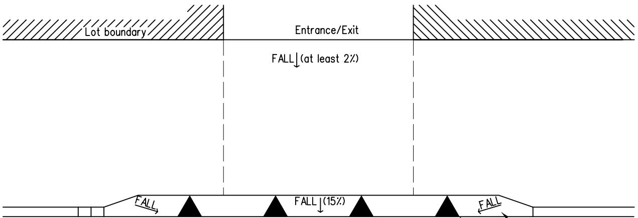
Road Markings of Levelled Run-in
