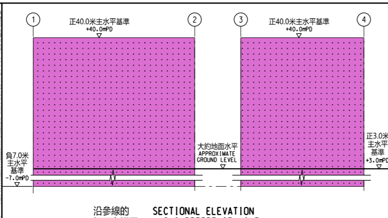
沿參線的 切面立視圖 SECTIONAL ELEVATION ALONG REFERENCE LINE SCALE HORI. 1:500 VERT. 1:100
