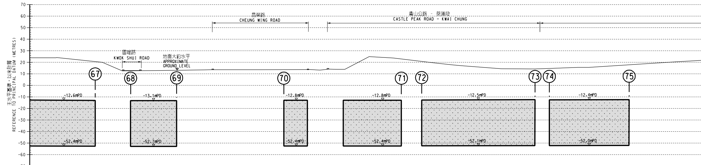
沿參線的切面立視圖 SECTIONAL ELEVATION ALONG REFERENCE LINE
